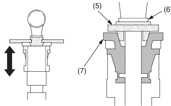
(5) joint rubber (injector side only) (6) flange (7) retainer tab
