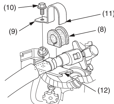
(8) setting rubber (9) clamp (10) bolt (11) clamp tab (12) groove
