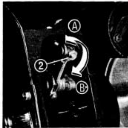
② Adjusting nut A Increase free play B Decrease free play
