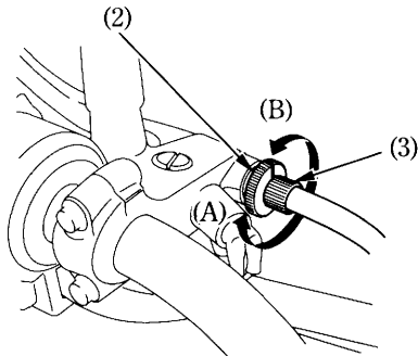
(2) Lock nut (A) Increase free play (3) Clutch cable adjuster (B) Decrease free play
