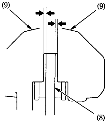
(8) Brake disc
