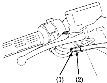
(1) Lock nut
