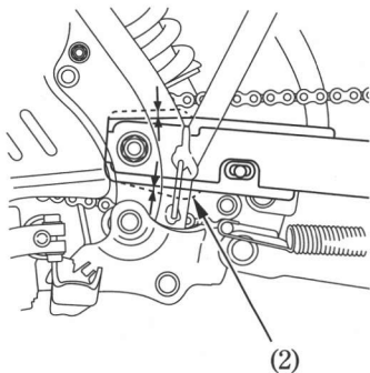
(2) Chain slider
