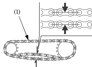
(1) Drive chain
