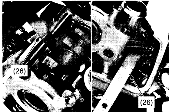
(26) feeler gauge
