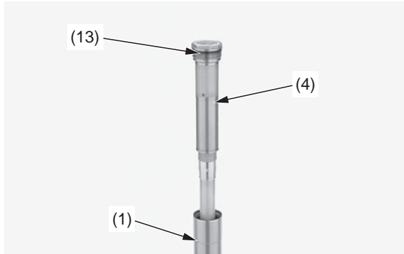
(1) fork assembly (13) O-ring (4) fork damper assembly
