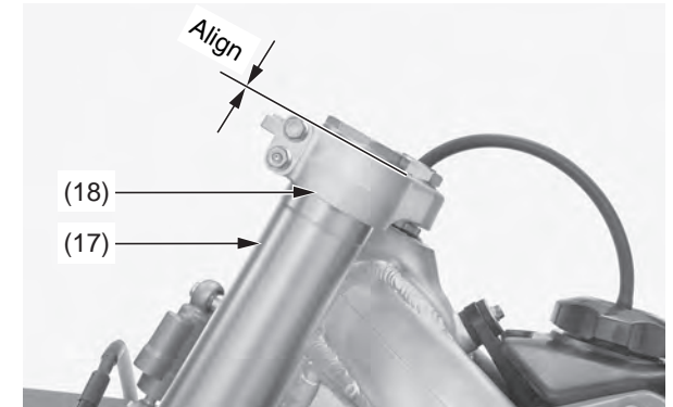
(17) outer tube (18) top bridge
