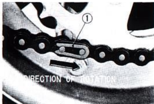
① Drive chain joint clip
