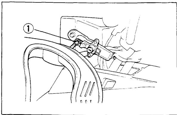
(1) Helmet holder
