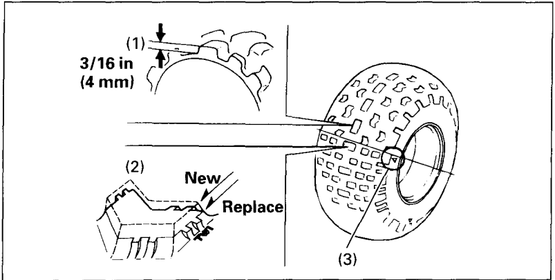
Fig. 4-29 (1) Groove depth (2) Wear indicator
