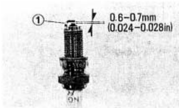
(1) Side electrode
