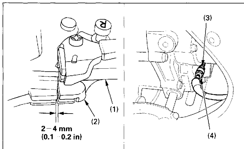
Fig. 4-16 (1) Rear brake lever (2) Reverse assist lever
