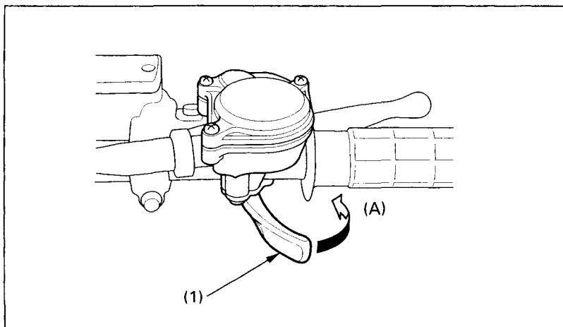
Fig. 2-10 (1) Throttle lever
