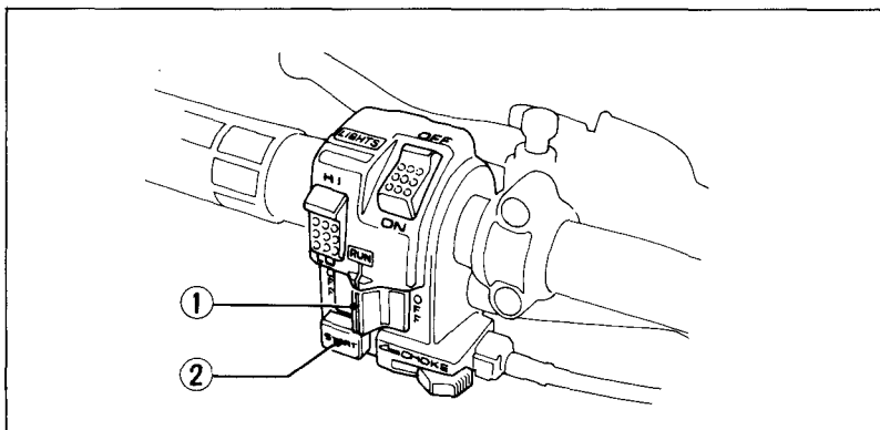
Fig. 2-5 (1) Engine stop switch (2) Starter button
