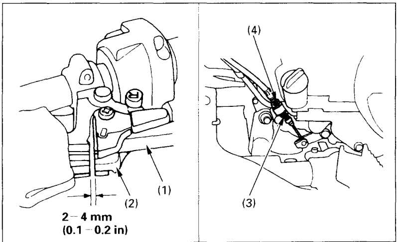
Fig. 4-19 (1) Rear brake lever (2) Reverse assist lever
