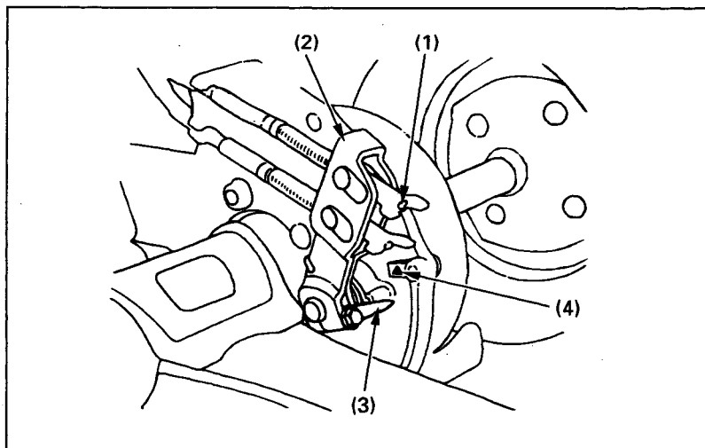
Fig. 4-28 (1) Brake lever adjusting nut (3) Arrow (2) Brake arm (4) Reference mark
