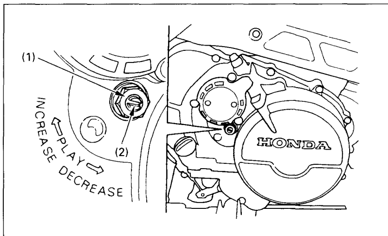
Fig. 4-17 (1) Lock nut
