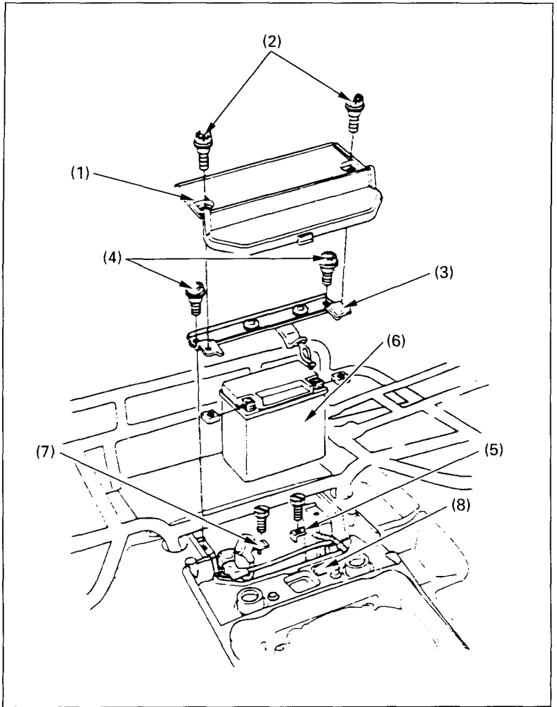
Fig. 4-19 (1) Battery box cover (2) Mount bolts (3) Battery holder (4) Mount bolts (5) Negative (-) terminal lead (6) Battery (7) Positive (+) terminal lead (8) Caution label
