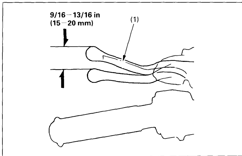
(1) Brake lever
