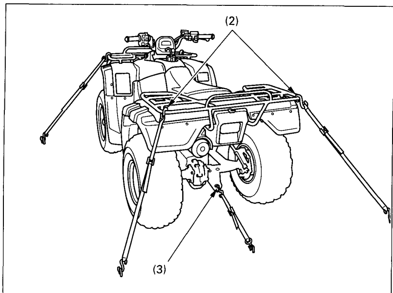
Fig. 4-43 Points to secure FOURTRAX with tie downs
