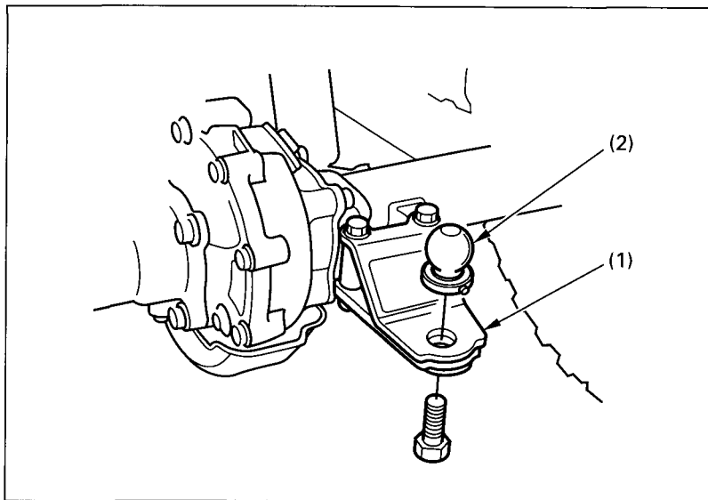
Fig. 2-30 (1) Trailer hitch
