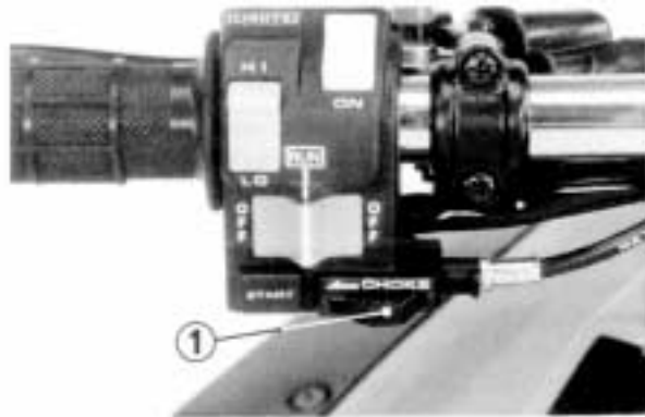
(1) Choke lever
