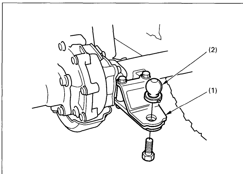
Fig. 2-30 (1) Trailer hitch
