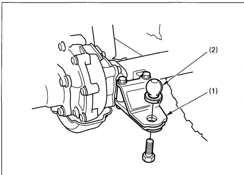
Fig. 2-29 (1) Trailer hitch
