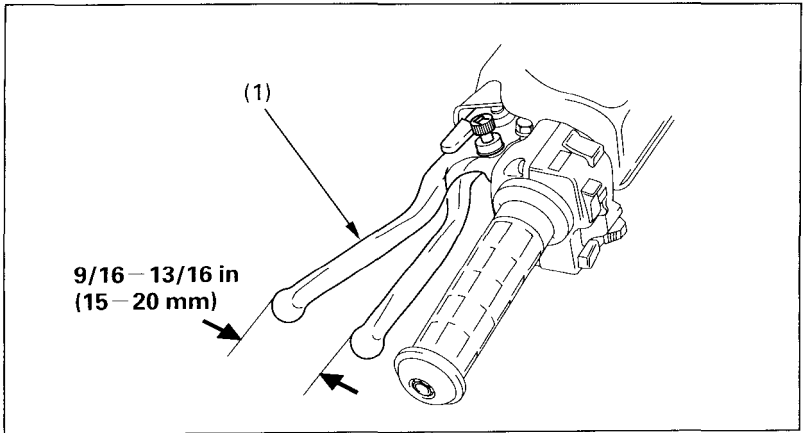
(1) Brake lever
