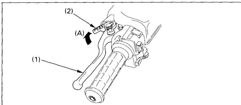
Fig. 2-17 (1) Rear brake lever/ Parking brake lever (2) Lock lever (A) To lock
