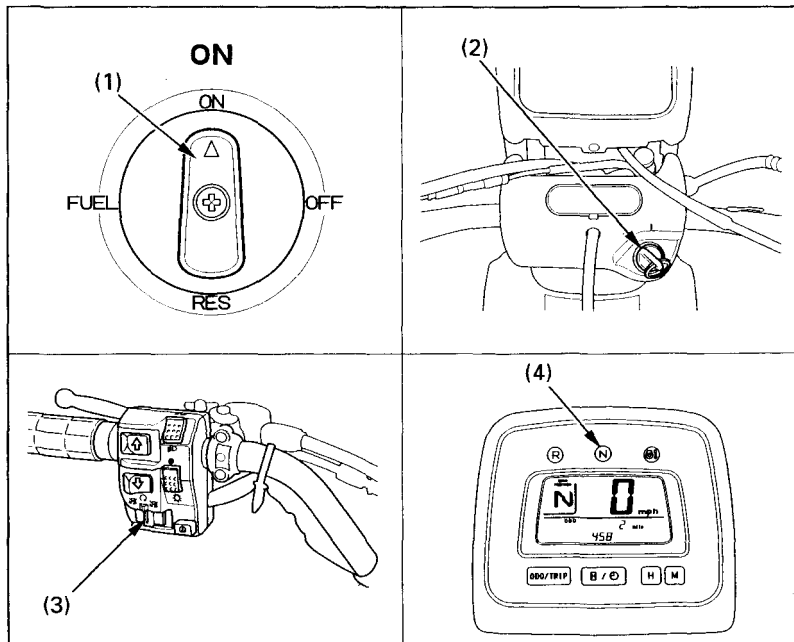
Fig. 3-9 (1) Fuel valve (2) Ignition switch
