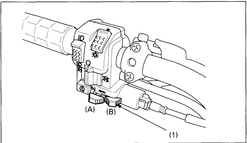
Fig. 2-7 (1) Choke lever
