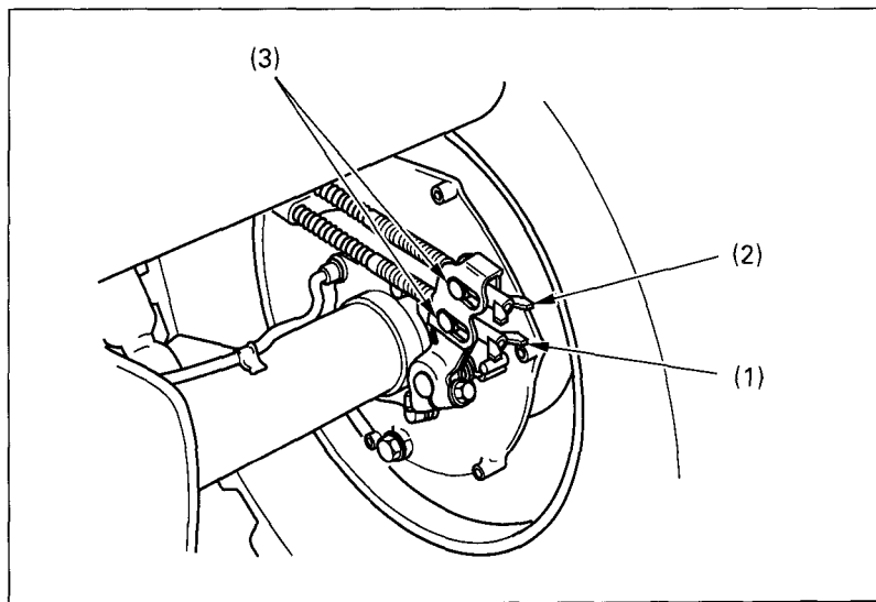
Fig. 4-28 (1) Brake pedal adjusting nut (2) Brake lever adjusting nut (3) Brake arm pin
