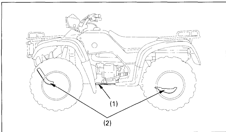
Fig. 4-37 (1) Engine guard
