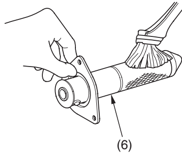
(6) spark arrester screen
