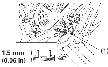
(1) chain roller
