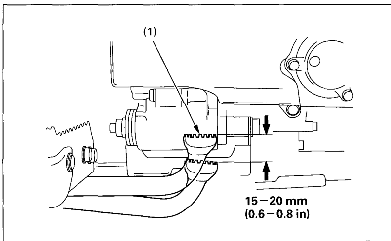
(1) Rear brake pedal
