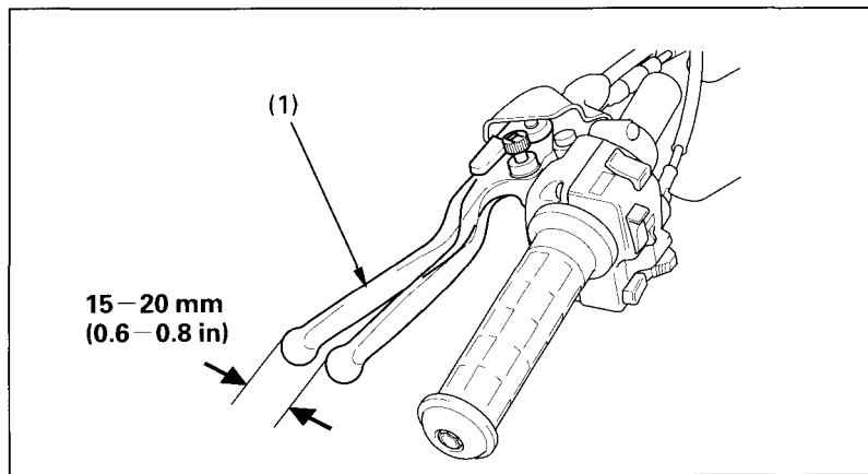
(1) Brake lever
