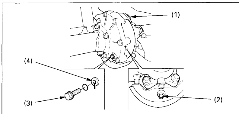
Fig. 4-16 (1) Oil filler cap (2) Drain plug (3) Oil level check bolt (4) Oil level check hole
