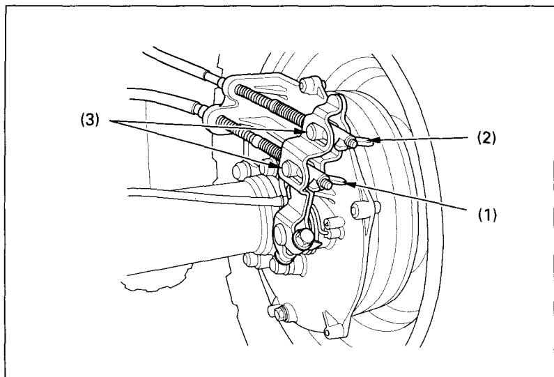
Fig. 4-31 (1) Brake pedal adjusting nut (2) Brake lever adjusting nut (3) Brake arm pin
