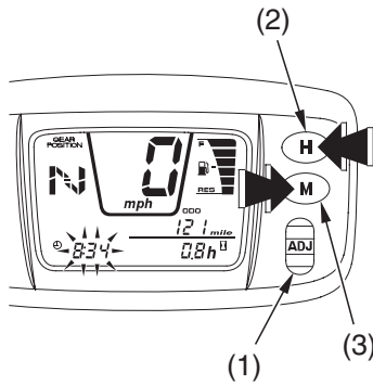
TRX500FE
