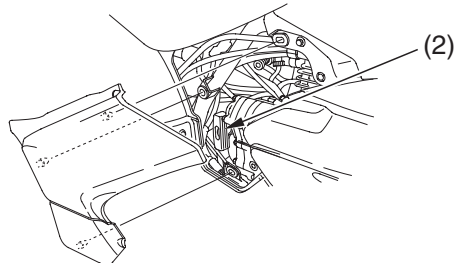
(2) recoil starter
