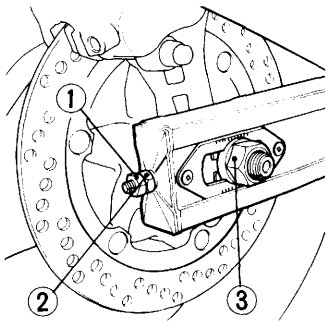
(1) Lock nuts
