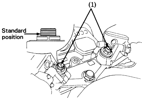
(1) Adjuster
