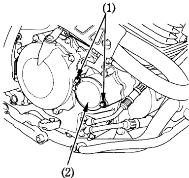
(2) Oil filter cover
