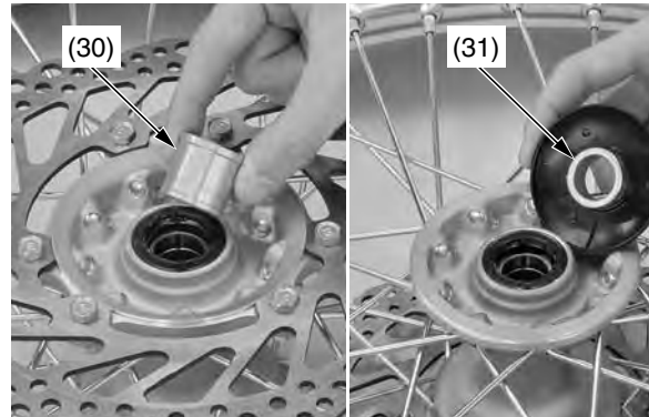
(30) left side collar (31) right side collar
