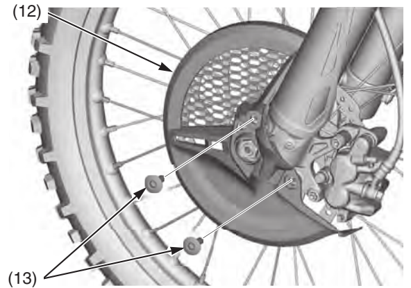
(12) disc cover (13) disc cover socket bolts
