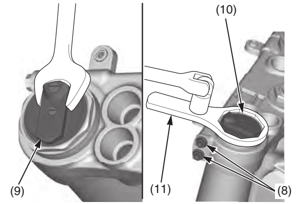
(8) fork bridge upper pinch bolts (9) fork bolt assembly (10) fork damper assembly (11) lock nut wrench
