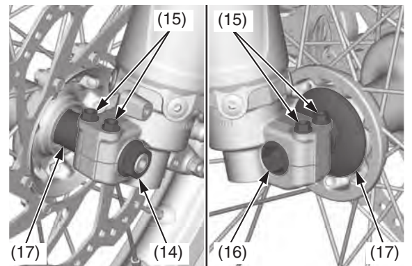
(14) front axle nut (16) front axle shaft (15) axle pinch bolts (17) collars
