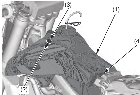
(1) fuel tank (2) collar (3) fuel tank bolt (4) fuel tank band
