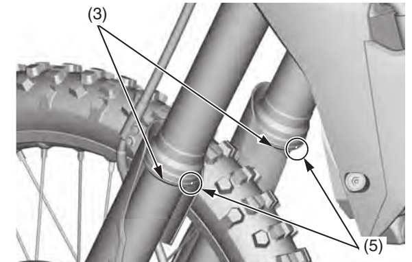
(3) wear rings
