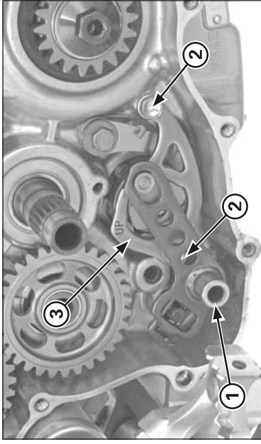
(1) GEARSHIFT SPINDLE (2) BOLTS (3) GUIDE PLATE
