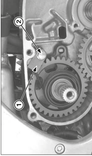
(1) STOPPER PLATE (2) BOLT
