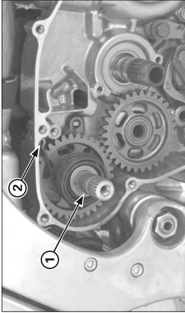
(1) KICKSTARTER ASSEMBLY (2) SPRING HOOK
