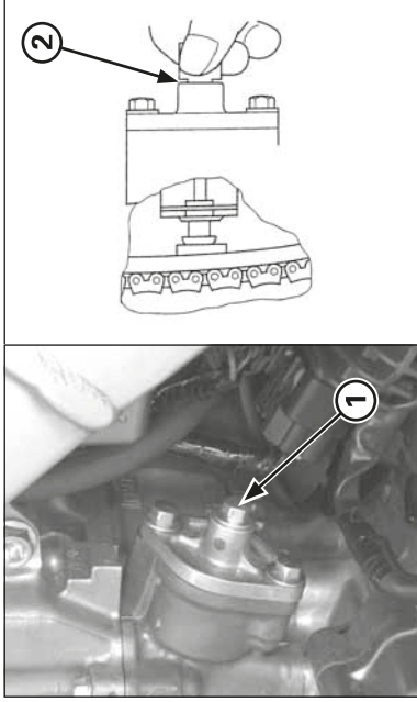
(1) SEALING BOLT/WASHER (2) STOPPER TOOL
