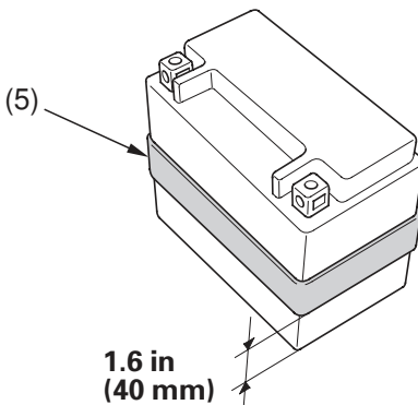
(5) battery band
